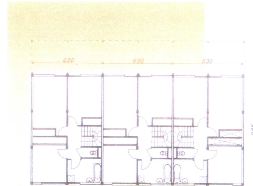
PLAN COMBLES
